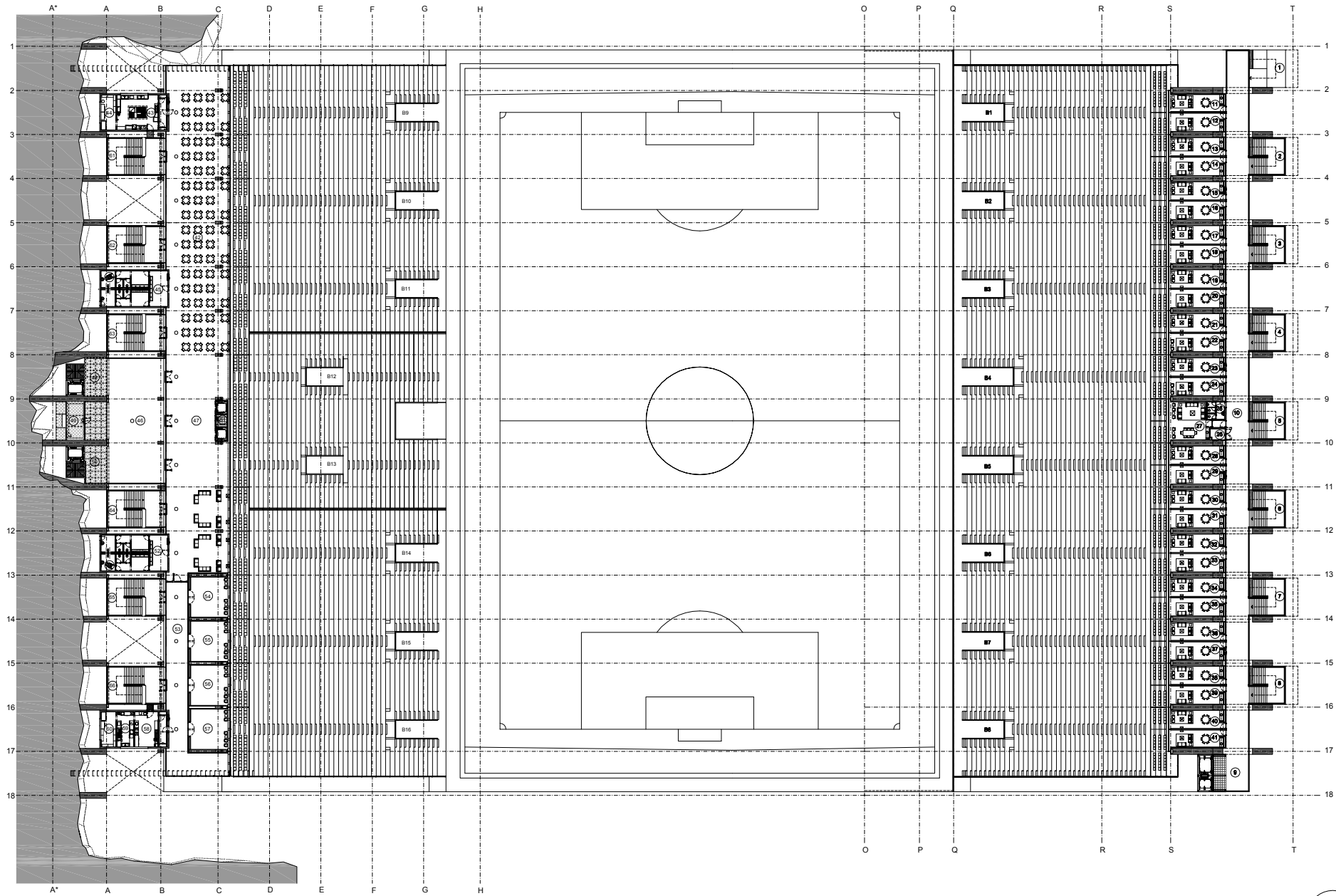
LEVEL 1 PLAN 0 10 20
